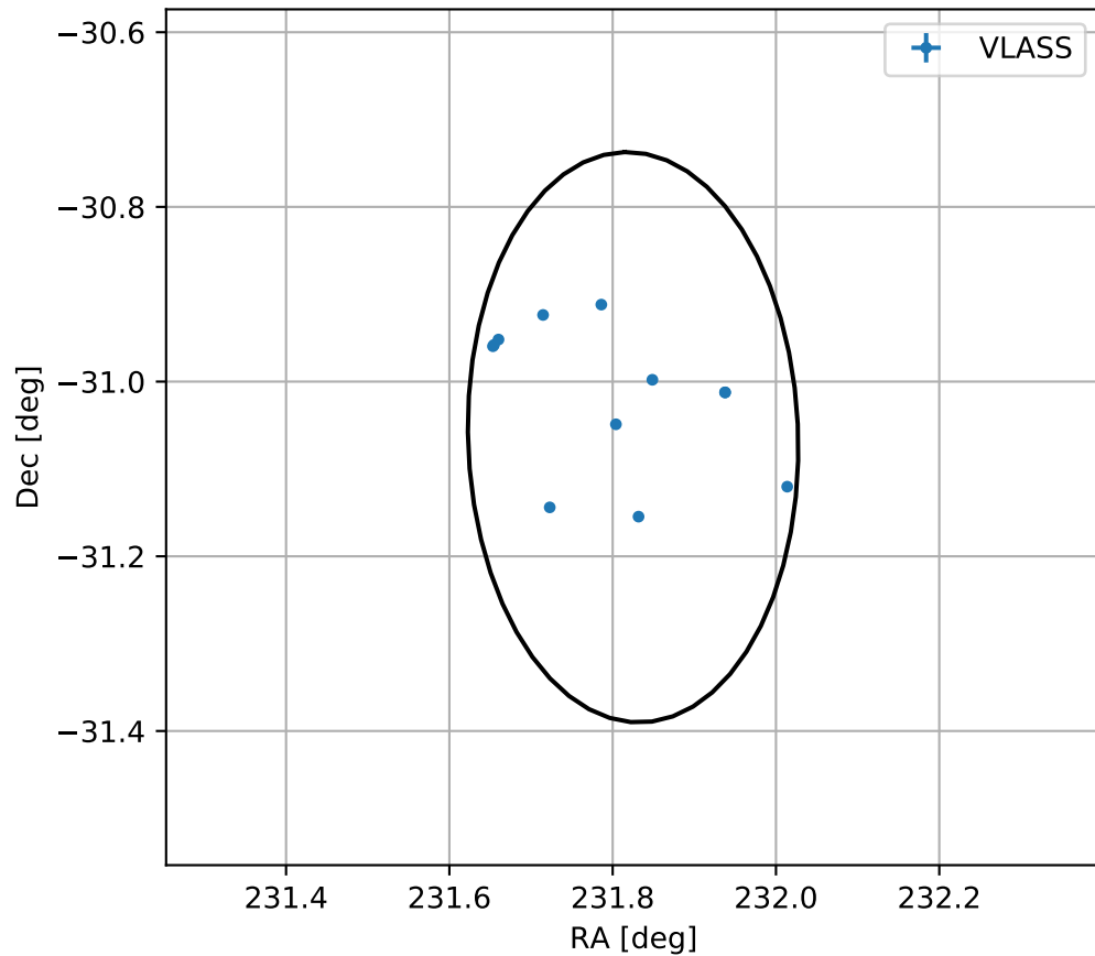
4FGL J1527.3-3103
