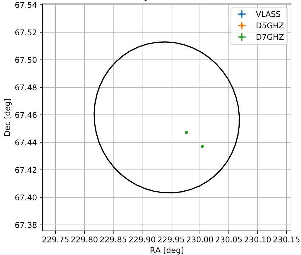
4FGL J1519.7+6727
