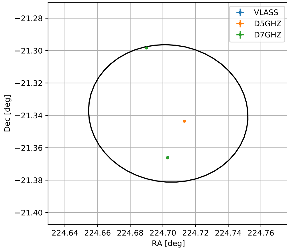
4FGL J1458.8-2120
