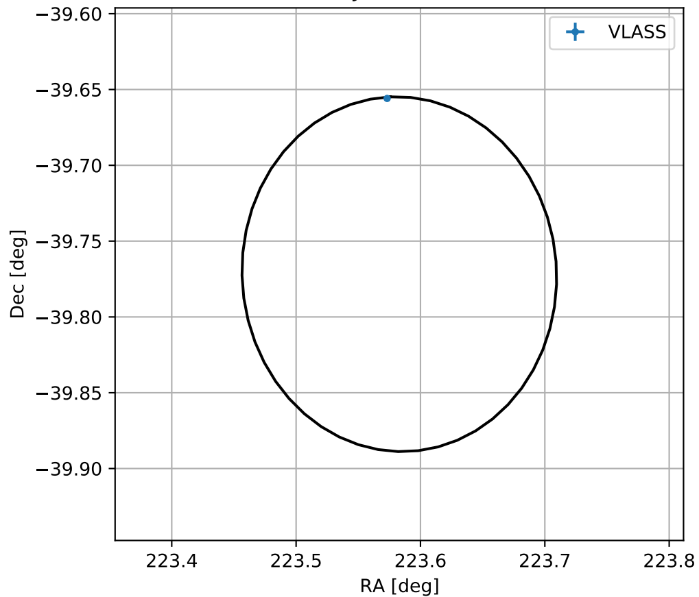
4FGL J1454.3-3946
