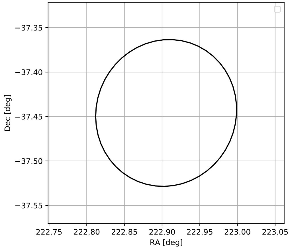
4FGL J1451.6-3726
