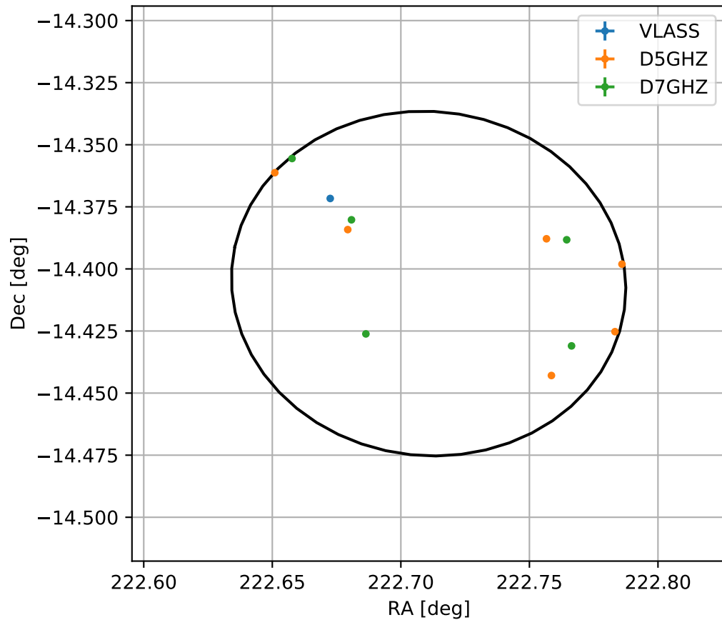
4FGL J1450.8-1424
