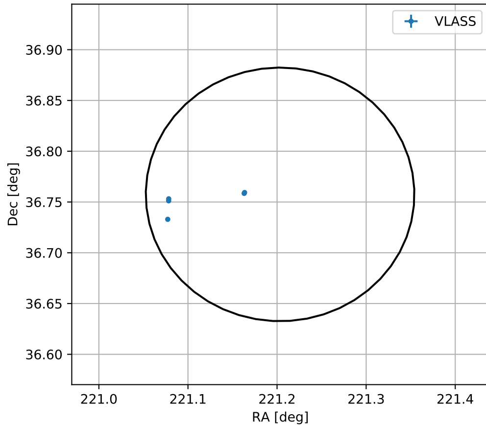
4FGL J1444.8+3645
