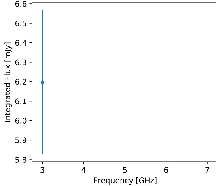
F357 J144439.25+364533.5 (res)
