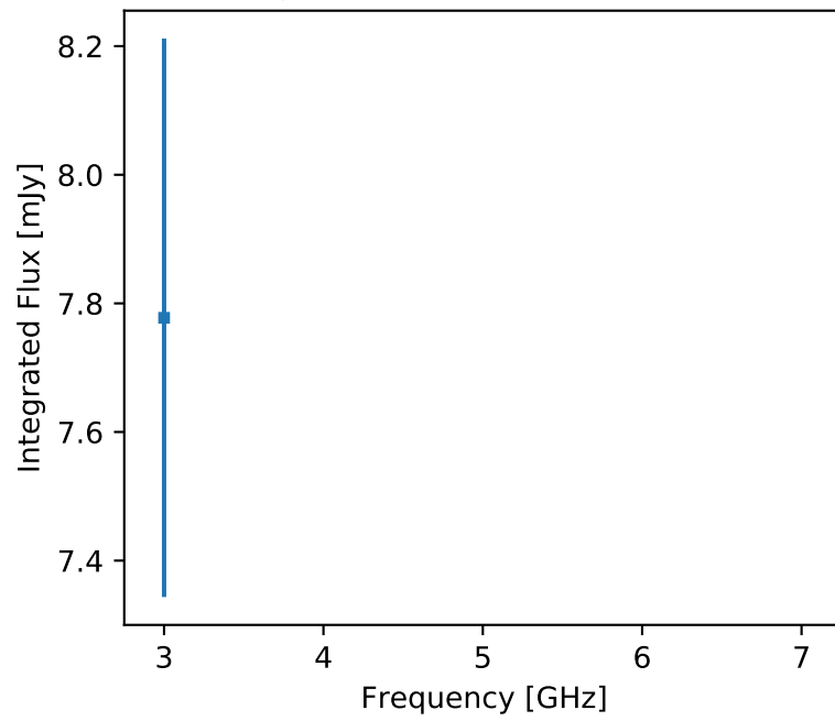
F357 J144418.81+364511.2 (res)
