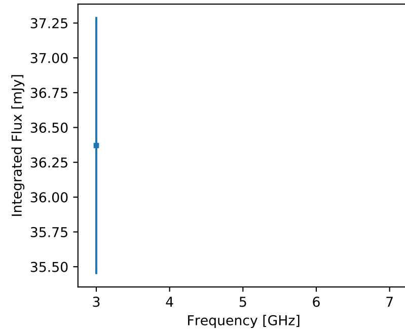
F357 J144439.25+364533.5 (res)
