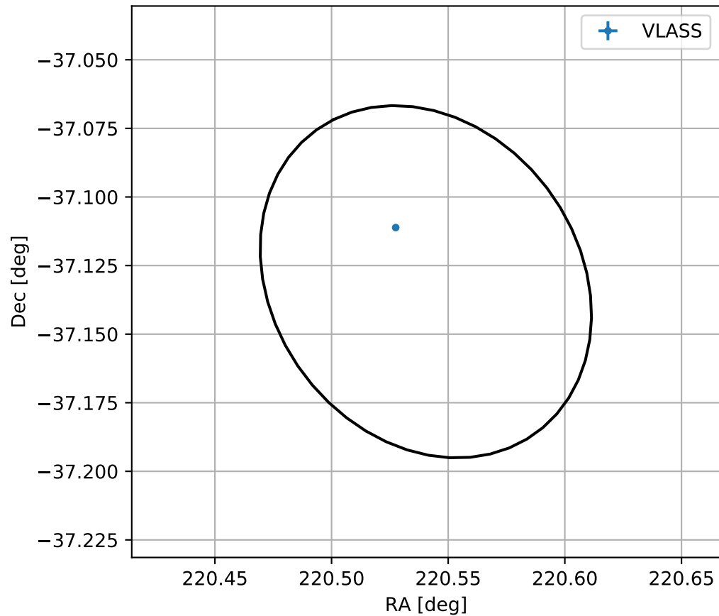
4FGL J1442.1-3707
