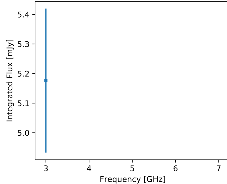
F357 J144206.59-370640.1 (unr)
