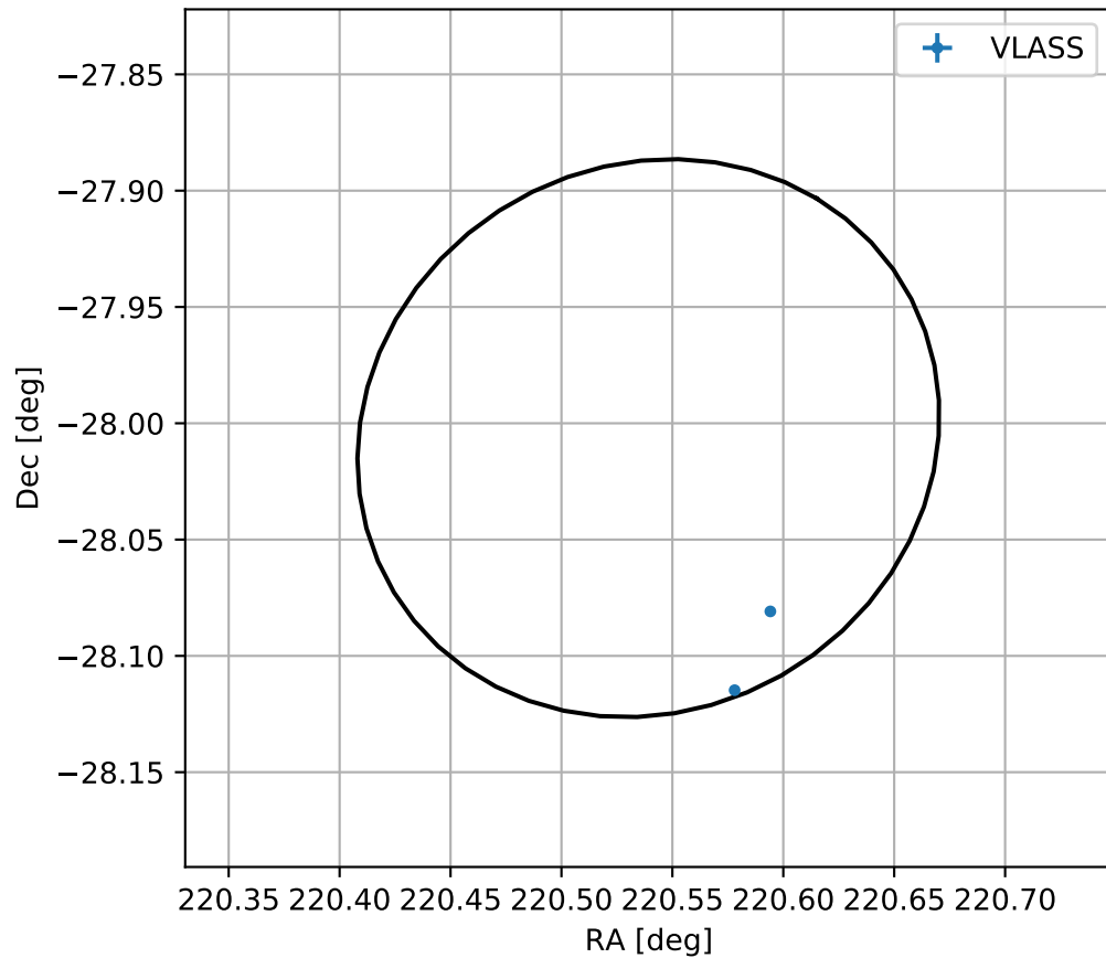
4FGL J1442.1-2800
