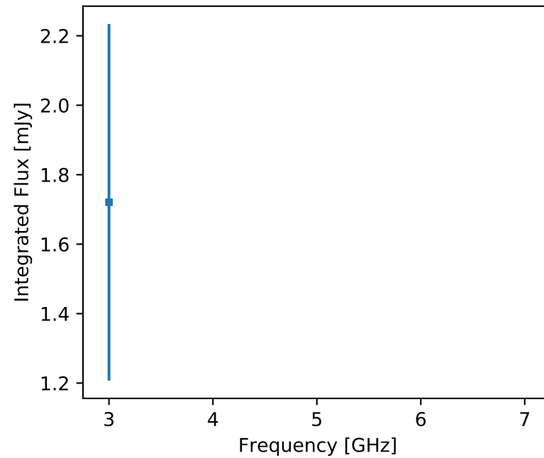
F357 J144222.60-280451.1 (unr)
