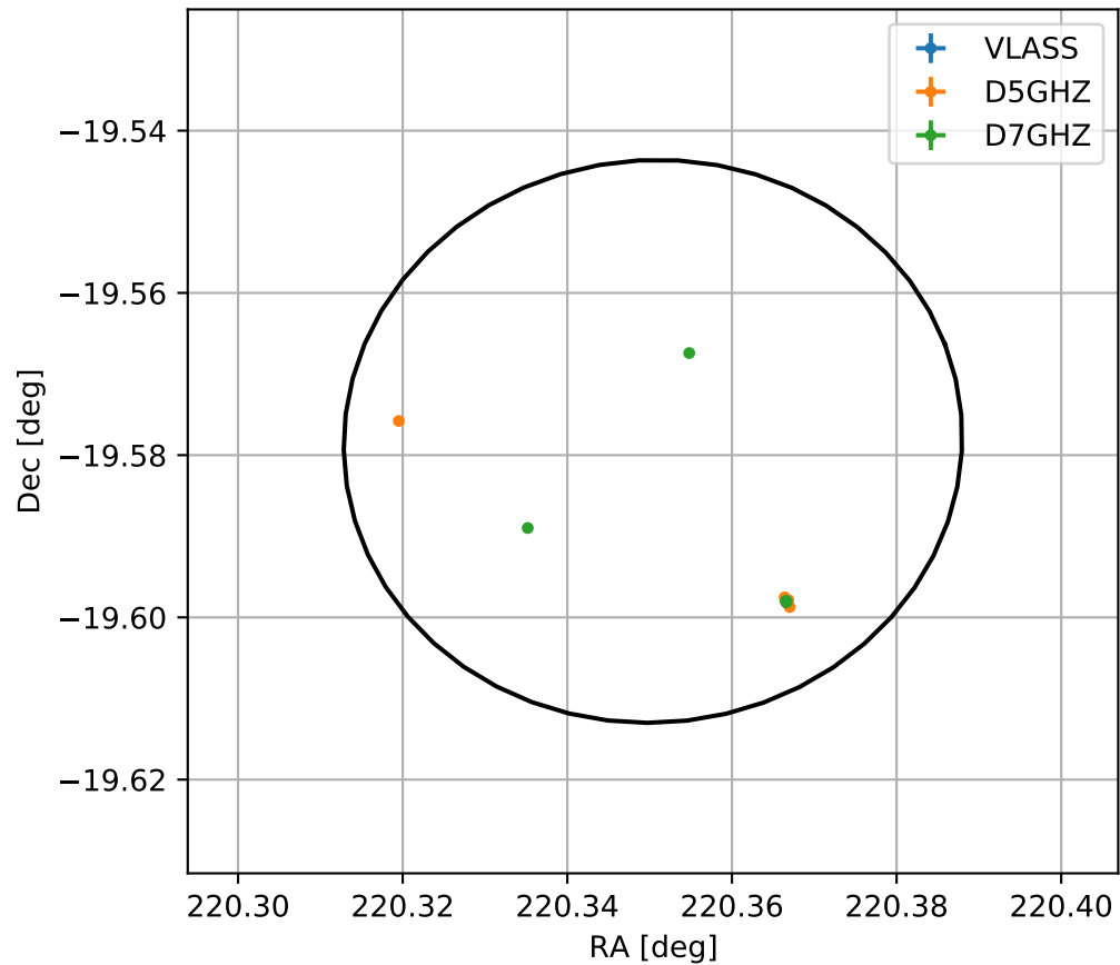
4FGL J1441.4-1934
