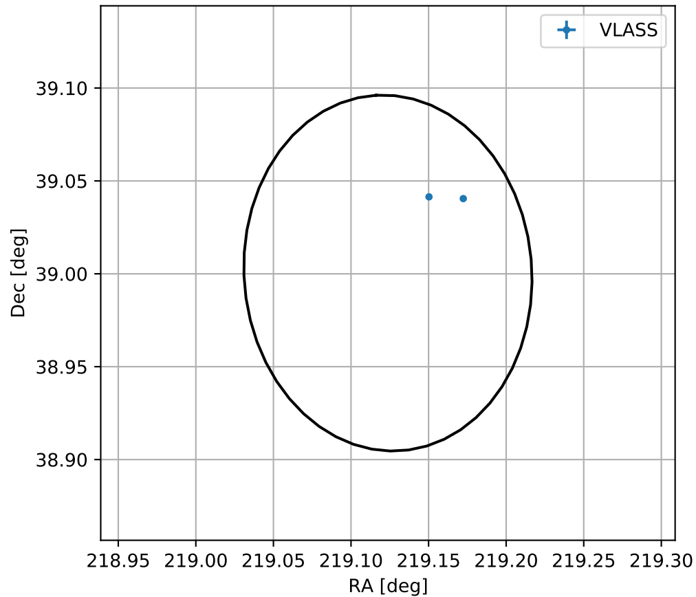
4FGL J1436.4+3900
