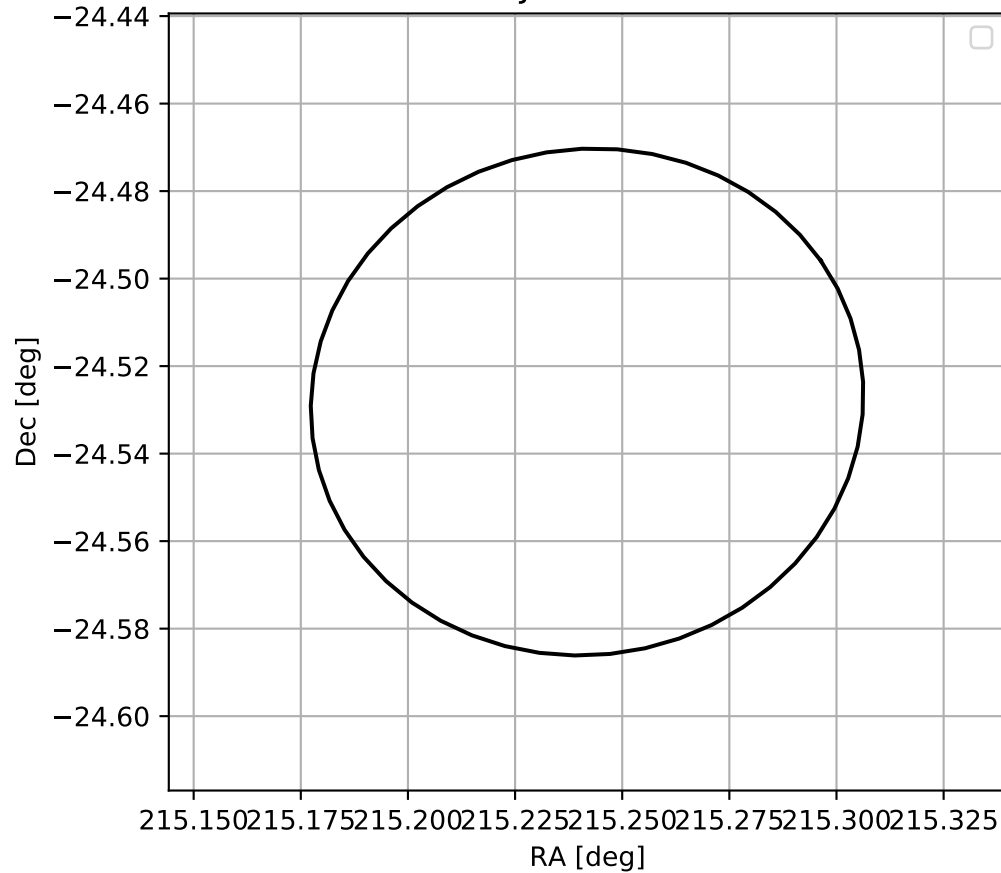
4FGL J1420.9-2431
