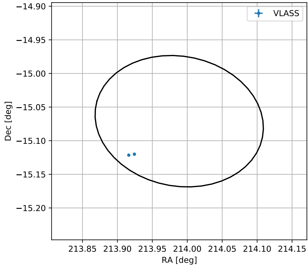
4FGL J1415.9-1504
