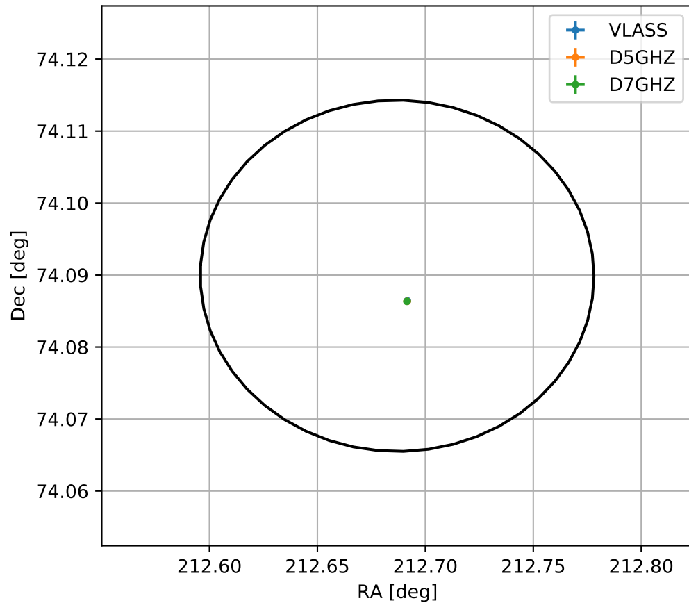
4FGL J1410.7+7405
