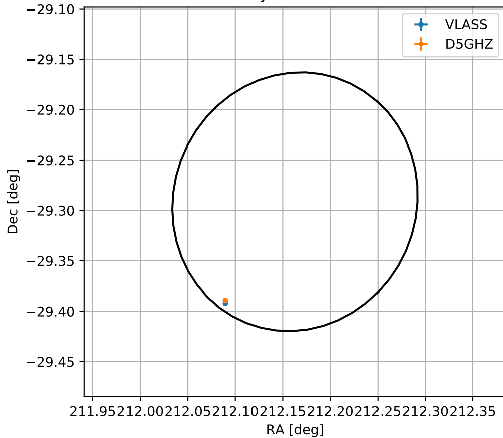
4FGL J1408.6-2917
