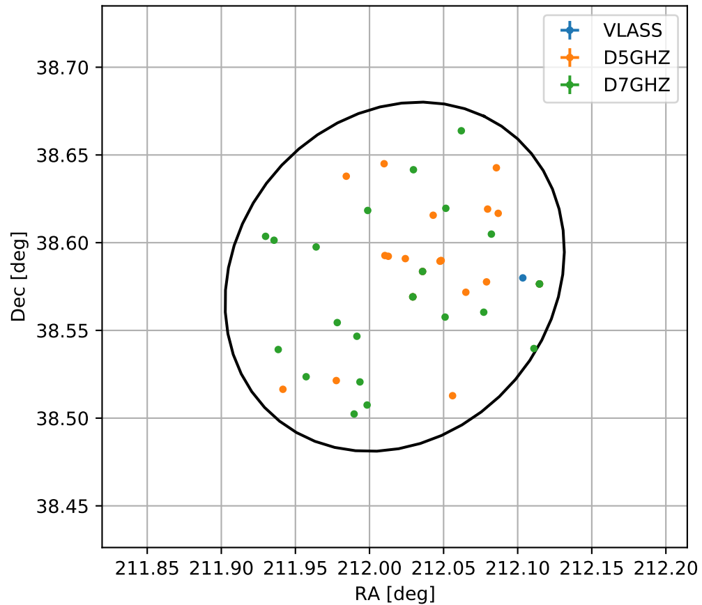
4FGL J1408.0+3834
