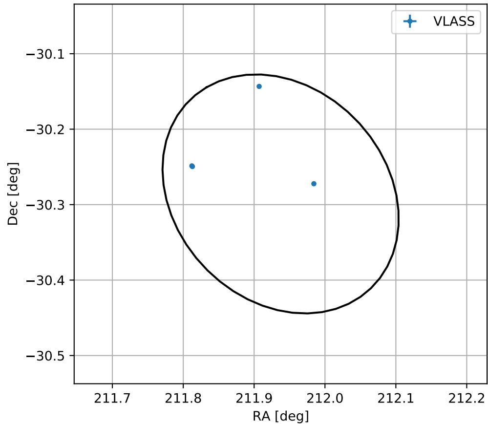
4FGL J1407.7-3017
