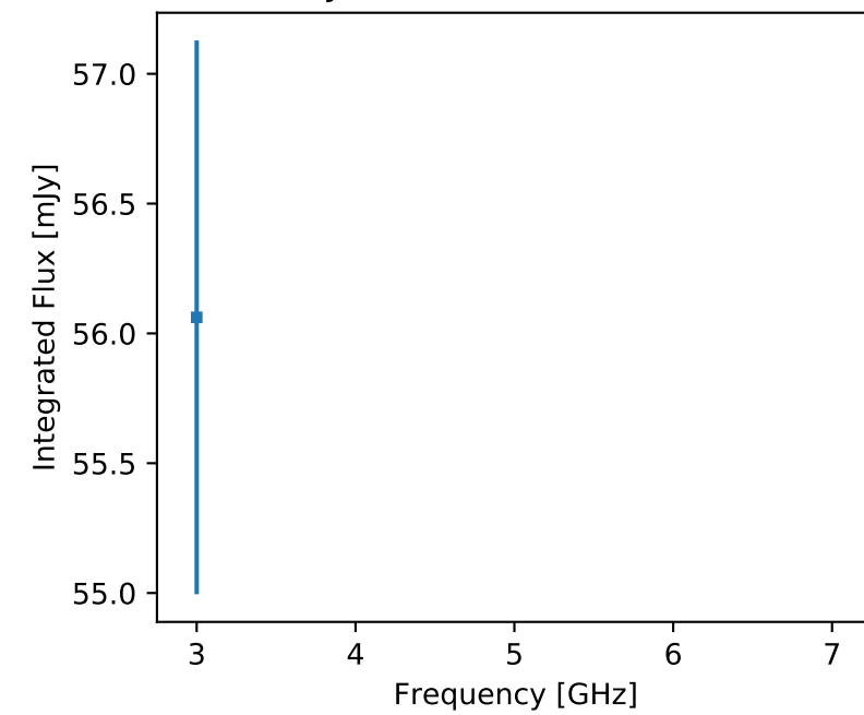
F357 J140737.70-300835.8 (unr)
