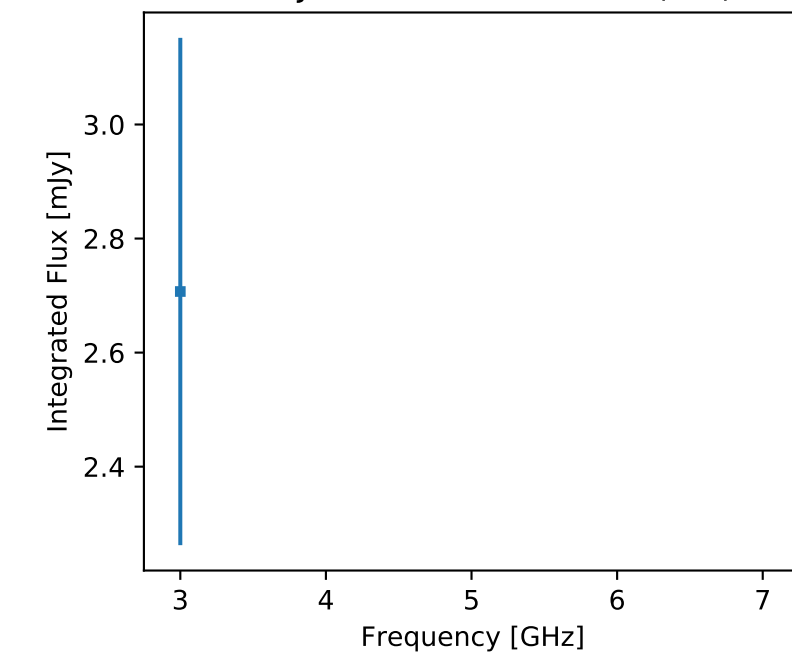
F357 J140756.23-301620.2 (unr)
