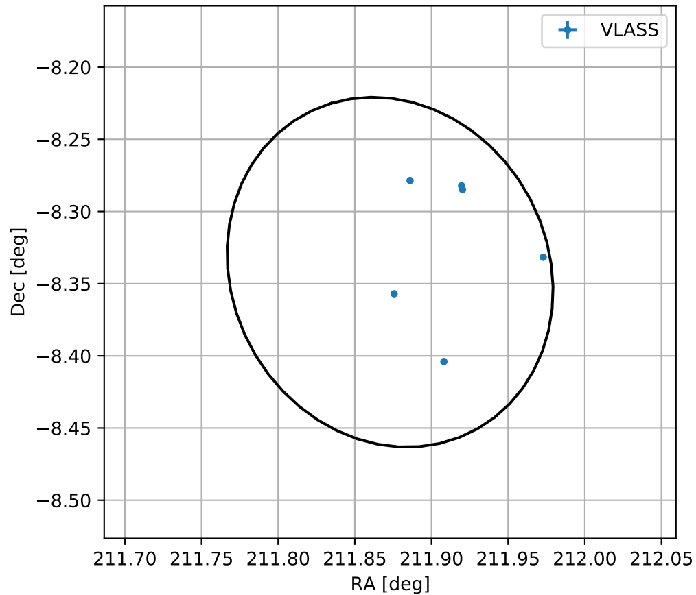
4FGL J1407.4-0820
