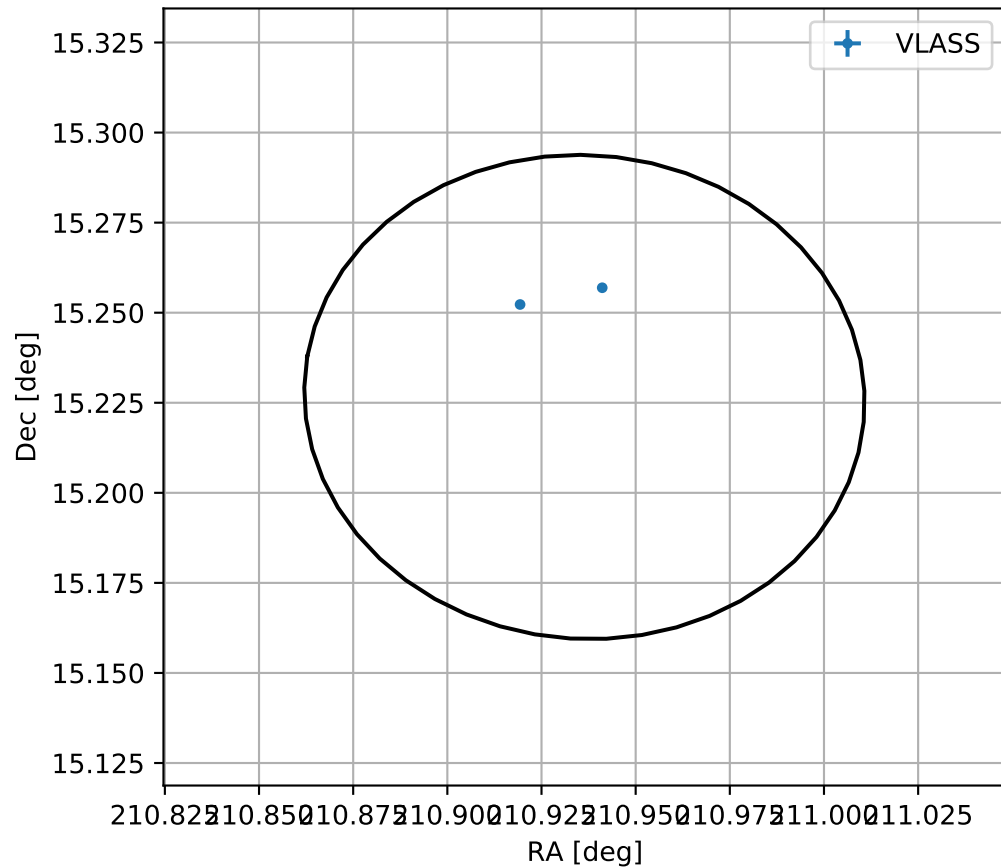
4FGL J1403.7+1513
