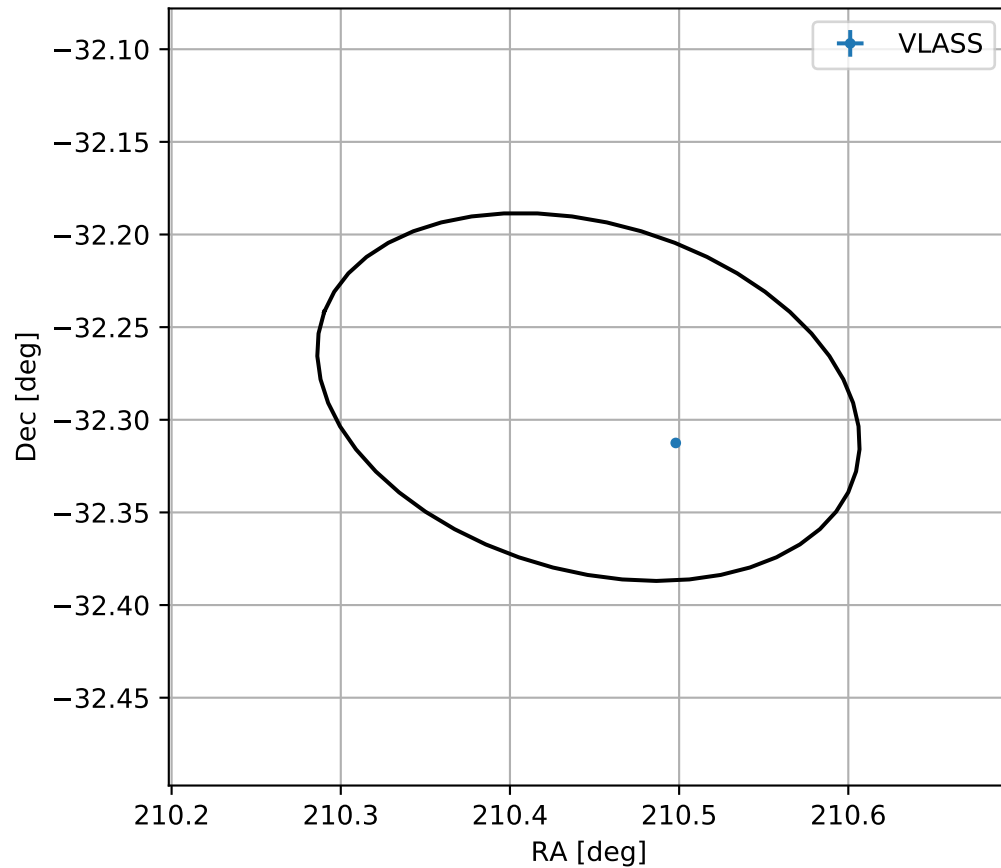
4FGL J1401.7-3217
