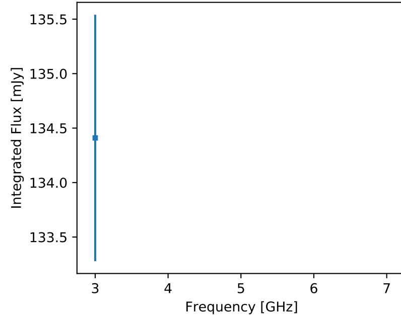
F357 J140159.51-321845.0 (unr)
