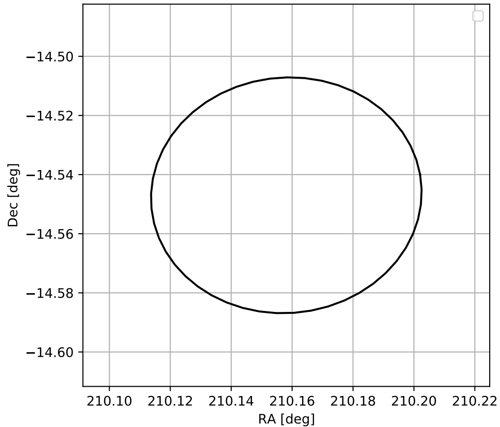
4FGL J1400.6-1432
