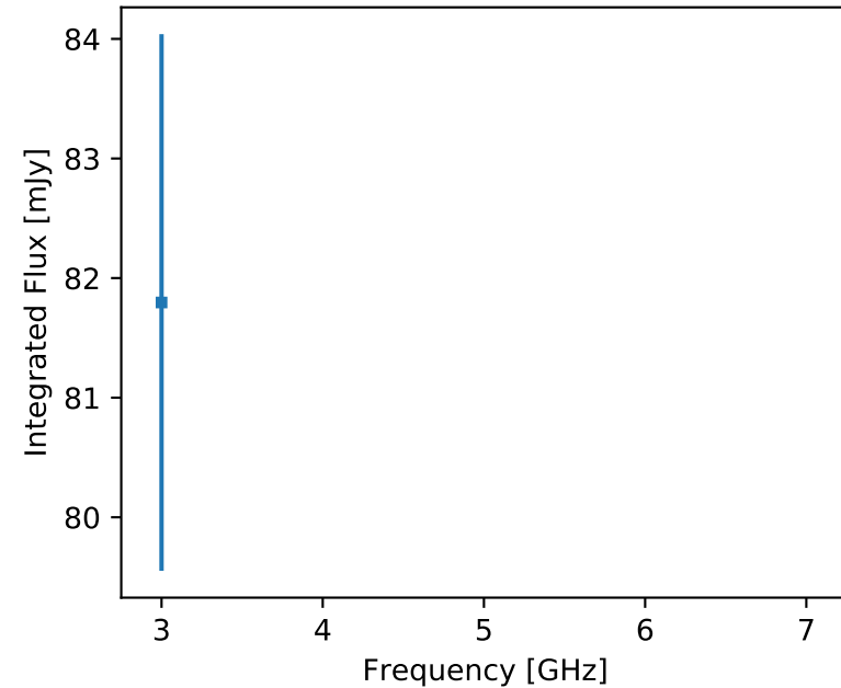
F357 J134600.42+532923.7 (res)
