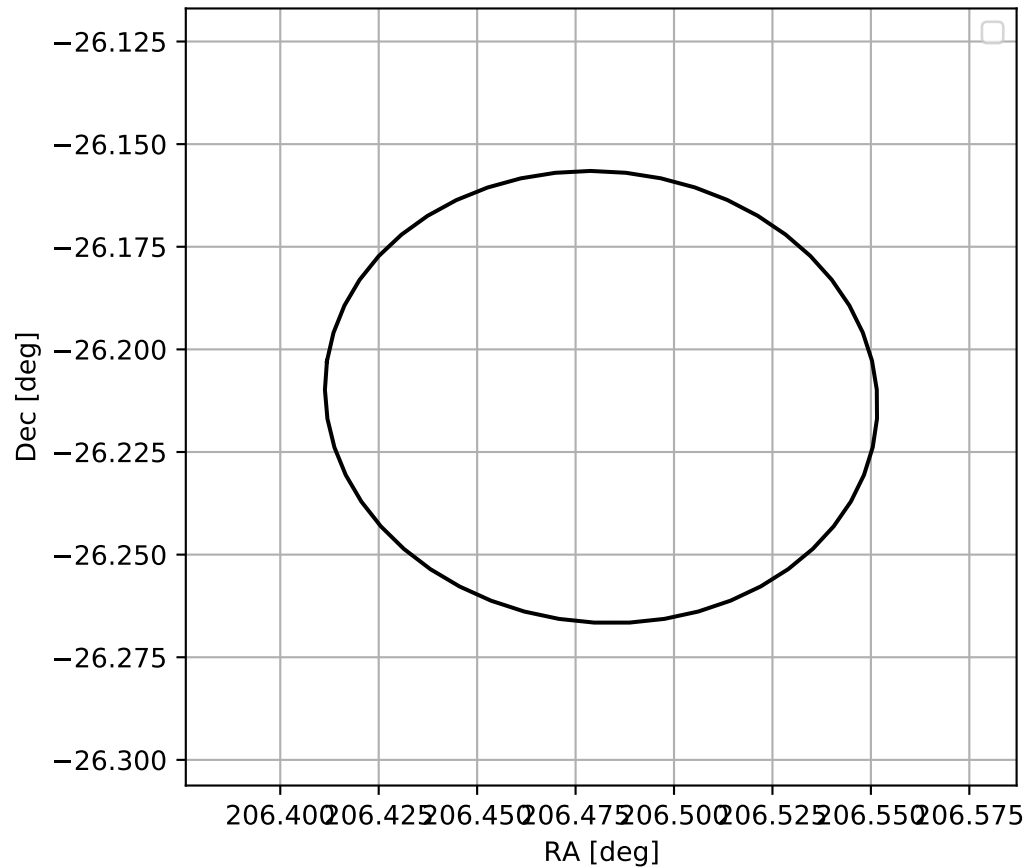
4FGL J1345.9-2612
