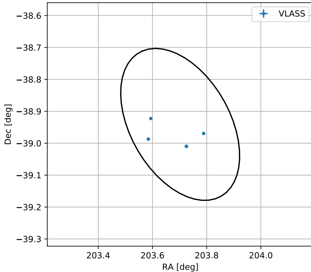
4FGL J1334.8-3856
