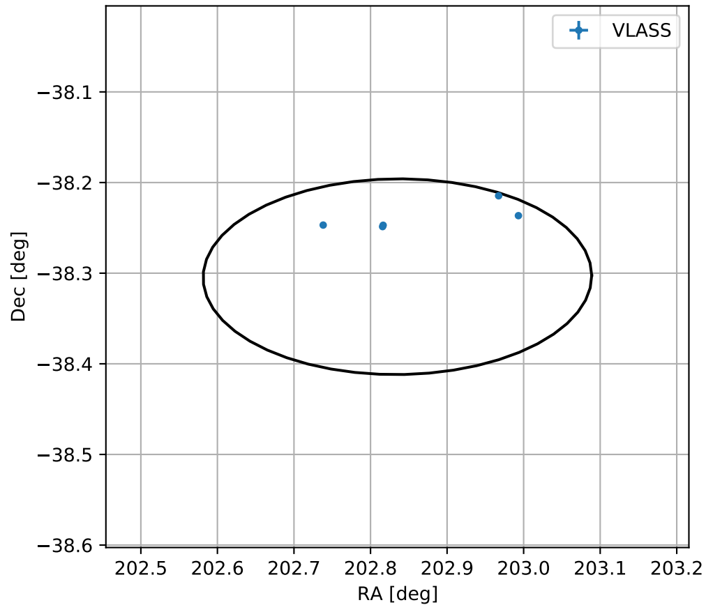
4FGL J1331.3-3818
