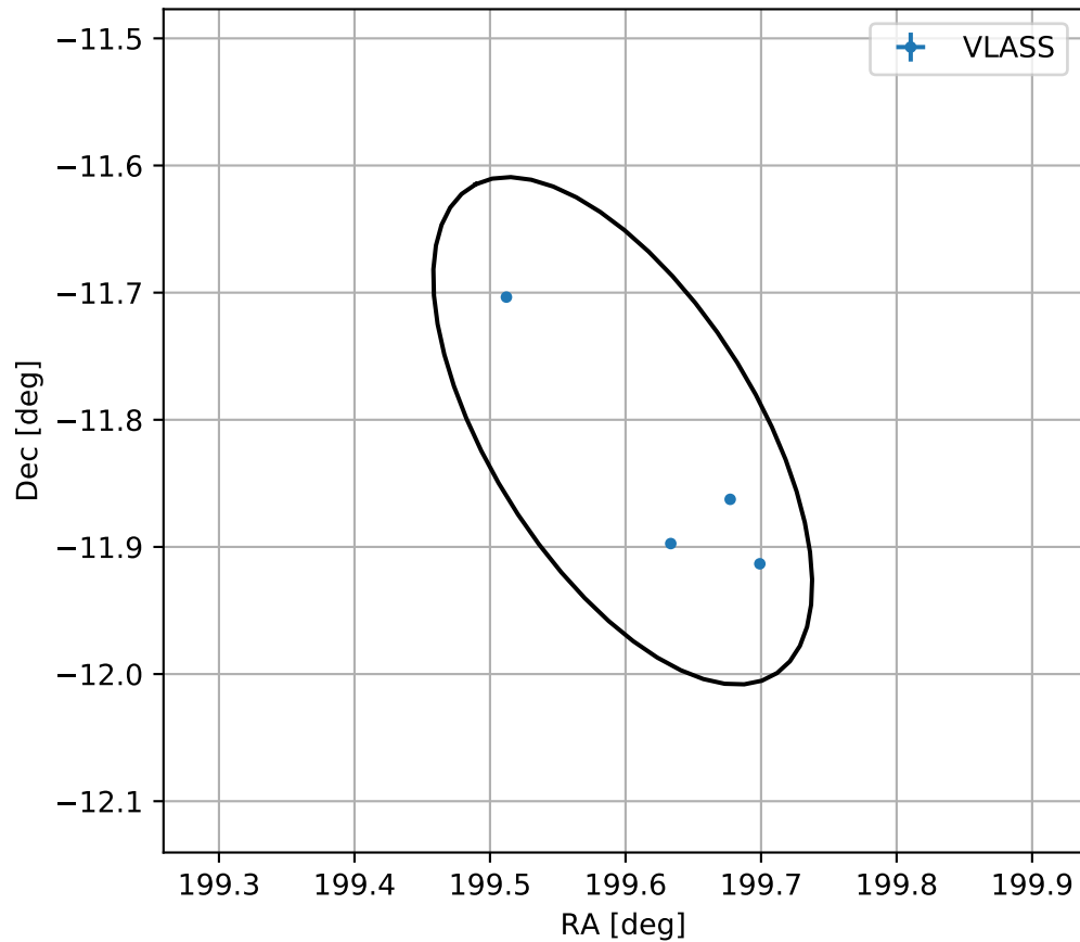
4FGL J1318.3-1148
