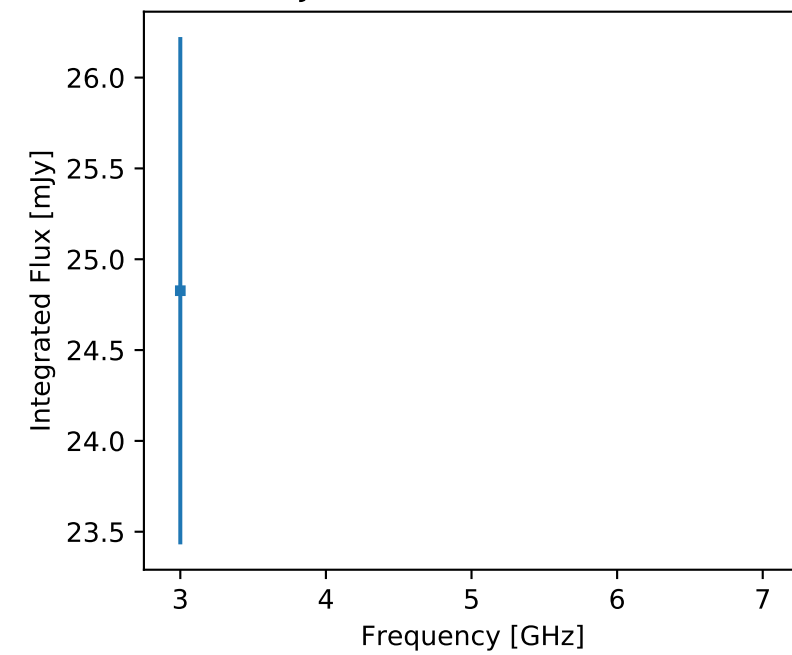
F357 J131818.68-393851.1 (unr)
