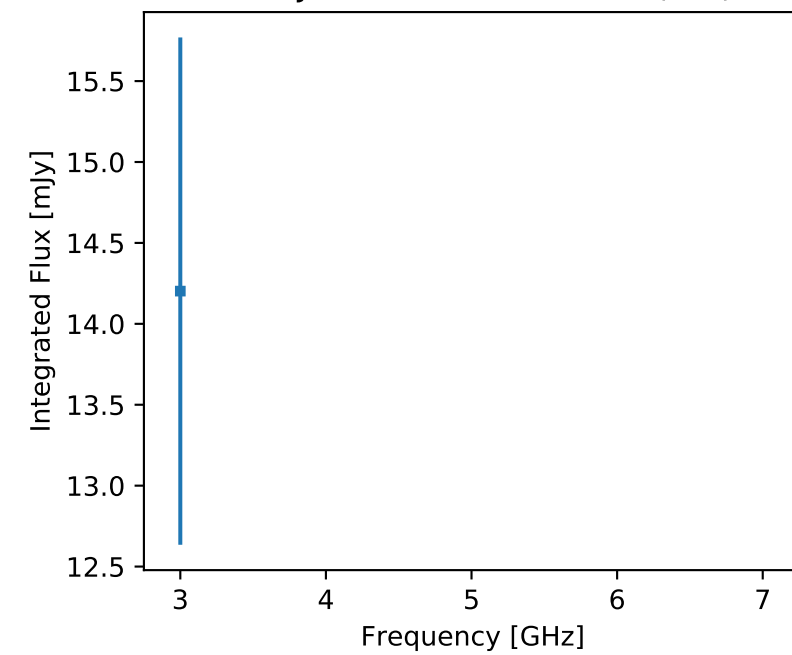
F357 J131818.80-393857.6 (unr)
