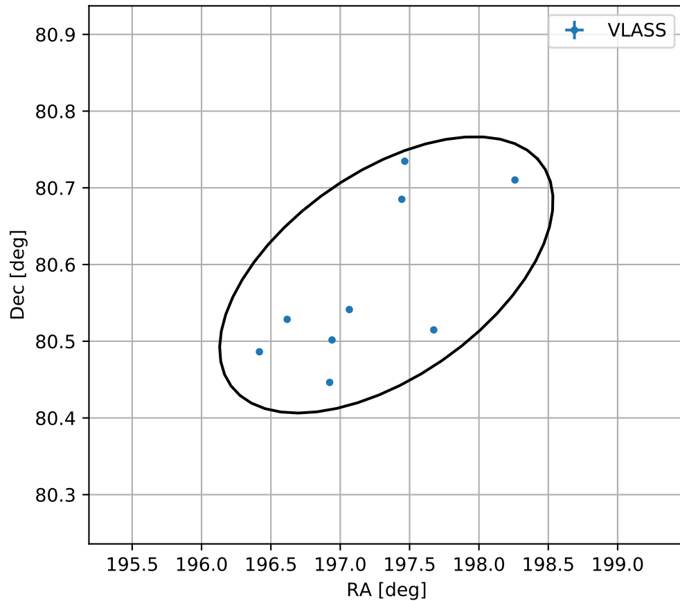
4FGL J1309.3+8035
