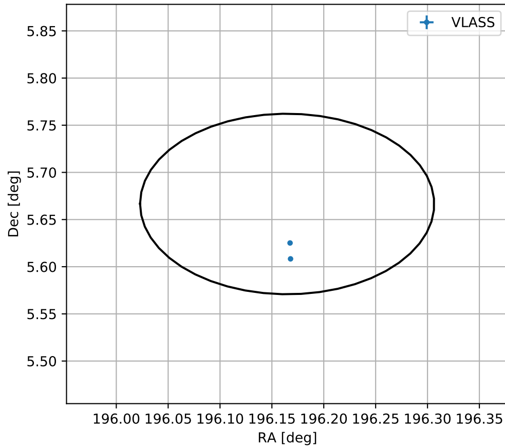
4FGL J1304.6+0539
