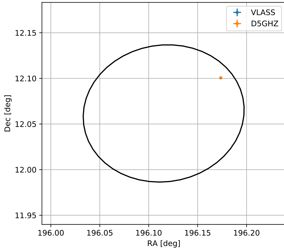
4FGL J1304.4+1203
