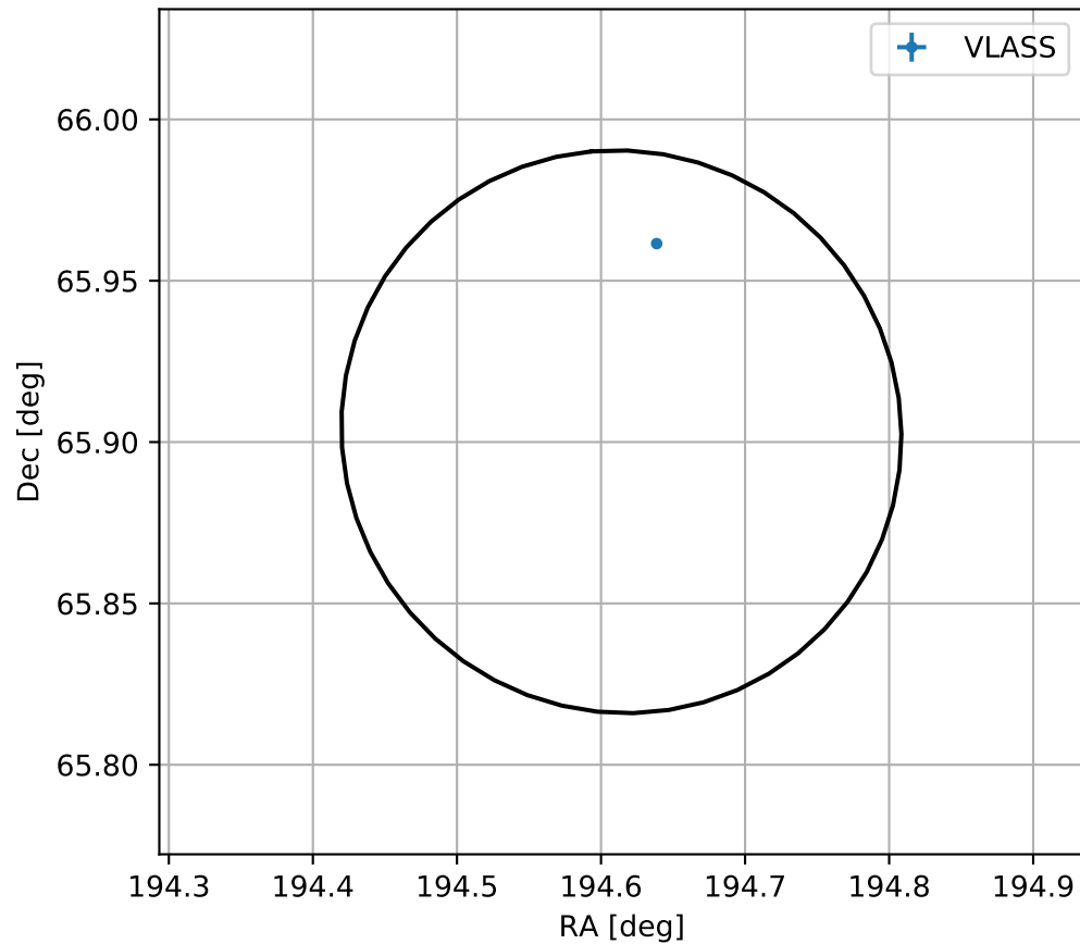
4FGL J1258.4+6554
