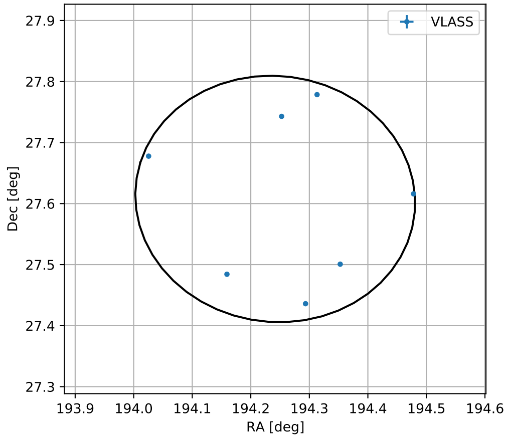
4FGL J1256.9+2736
