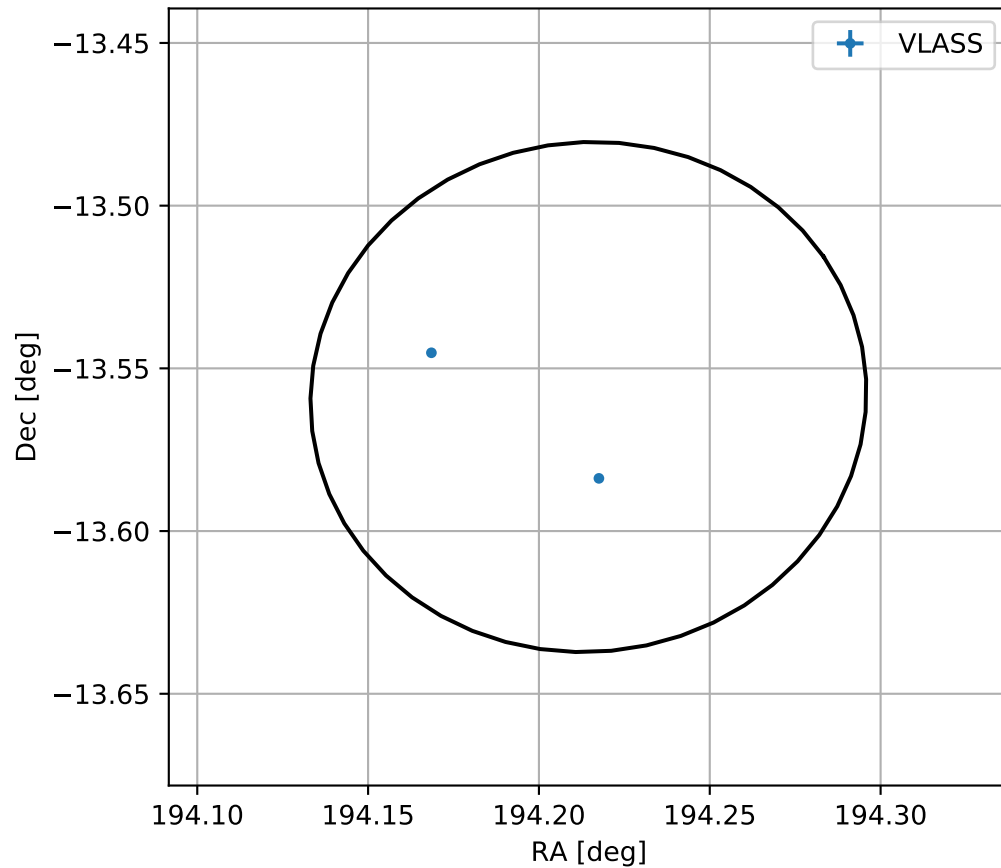
4FGL J1256.8-1333
