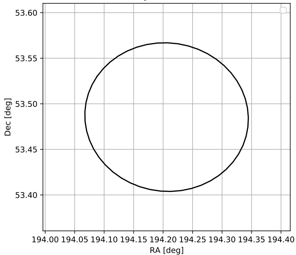
4FGL J1256.8+5329
