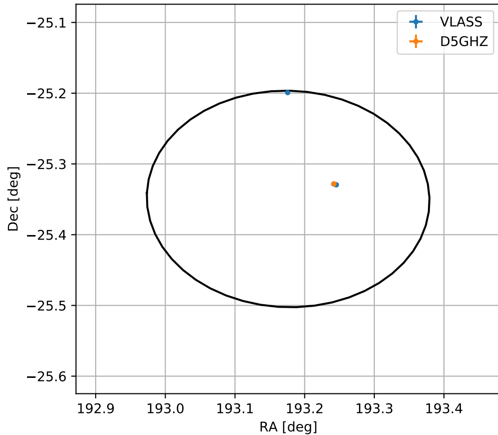
4FGL J1252.7-2520
