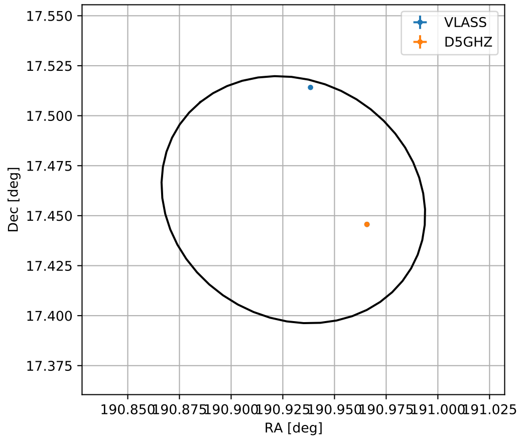
4FGL J1243.7+1727
