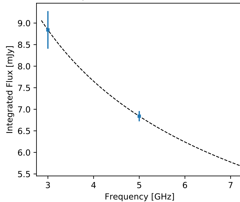
F357 J124351.76+172644.3 (unr)
