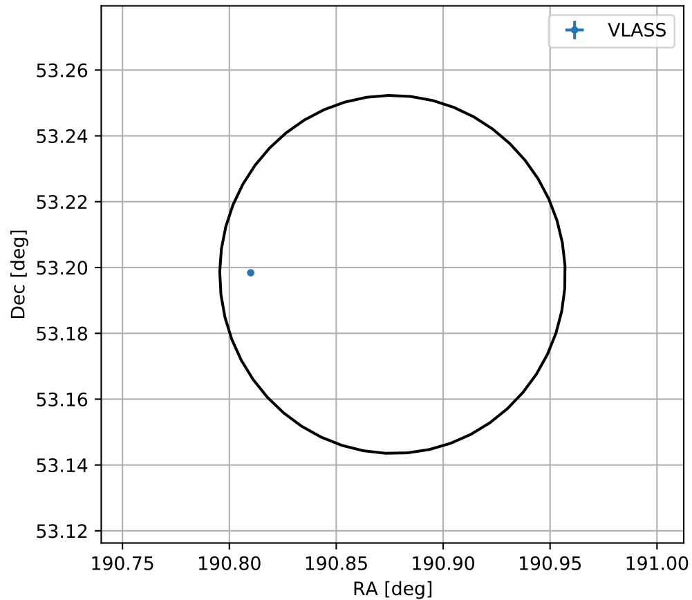
4FGL J1243.5+5311
