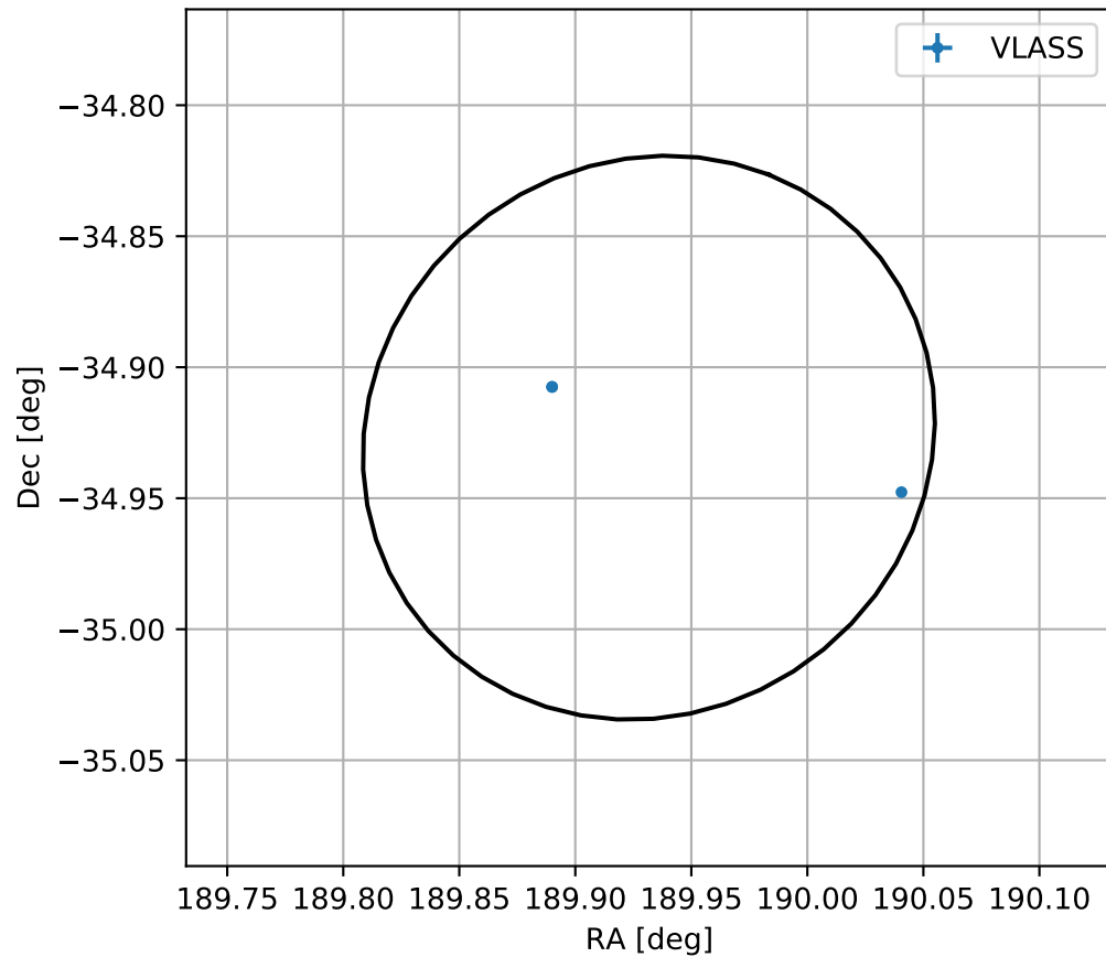
4FGL J1239.7-3455
