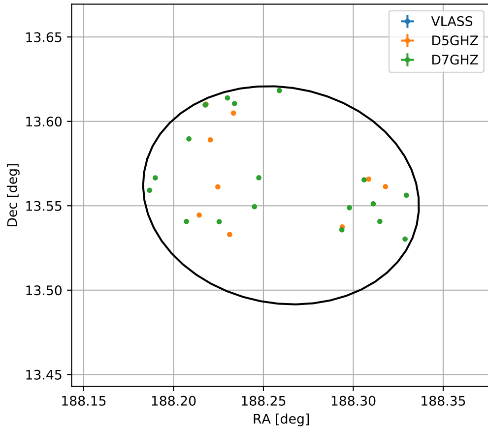
4FGL J1233.0+1333
