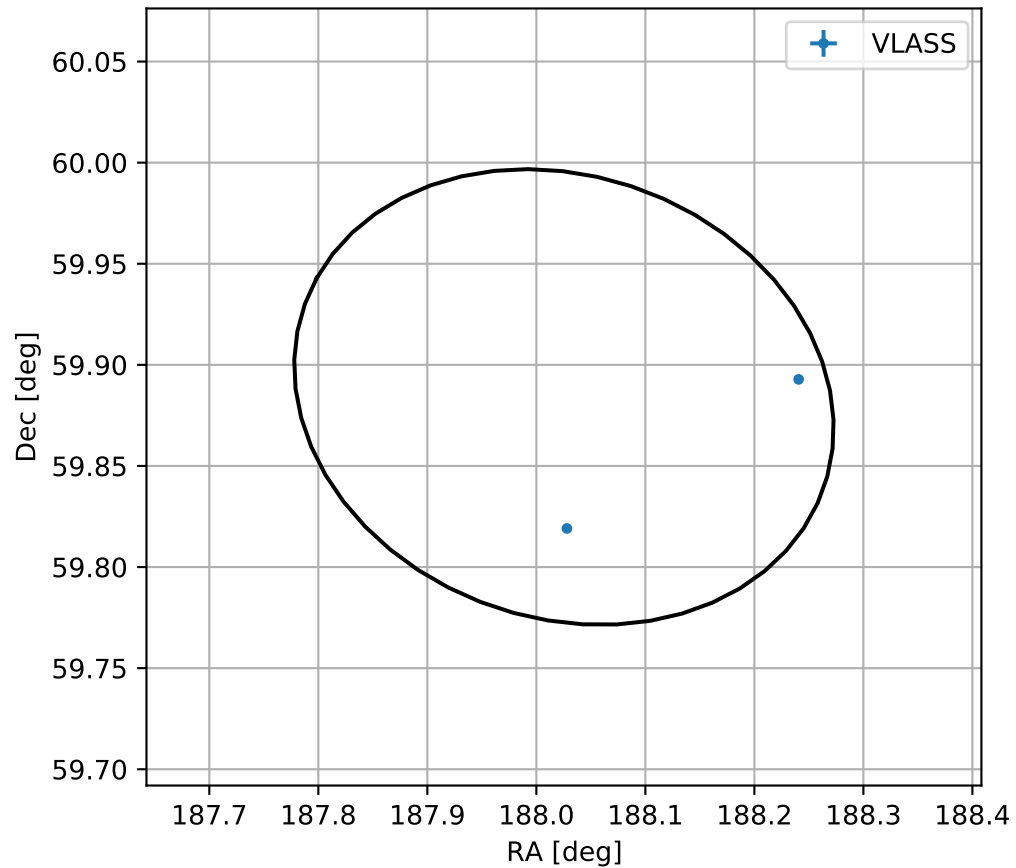
4FGL J1232.1+5953
