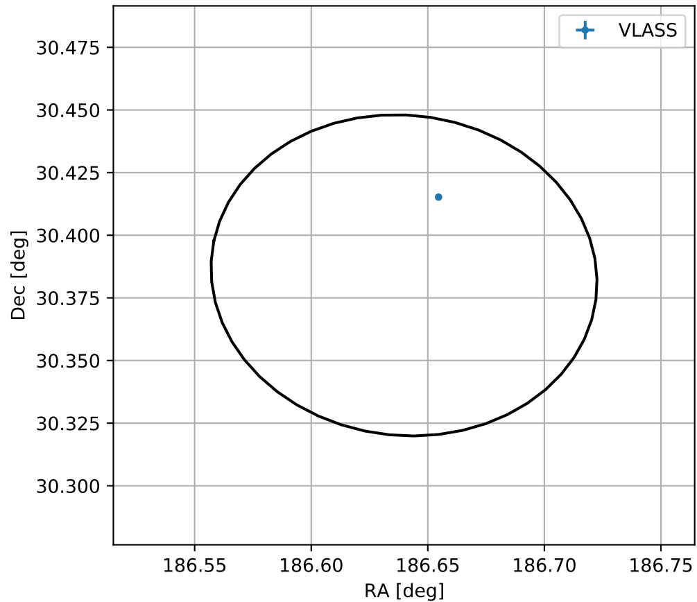
4FGL J1226.5+3023
