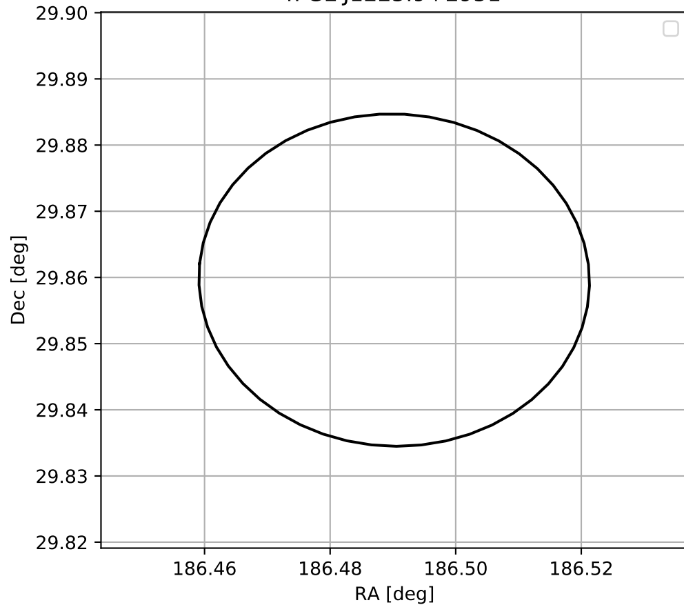
4FGL J1225.9+2951
