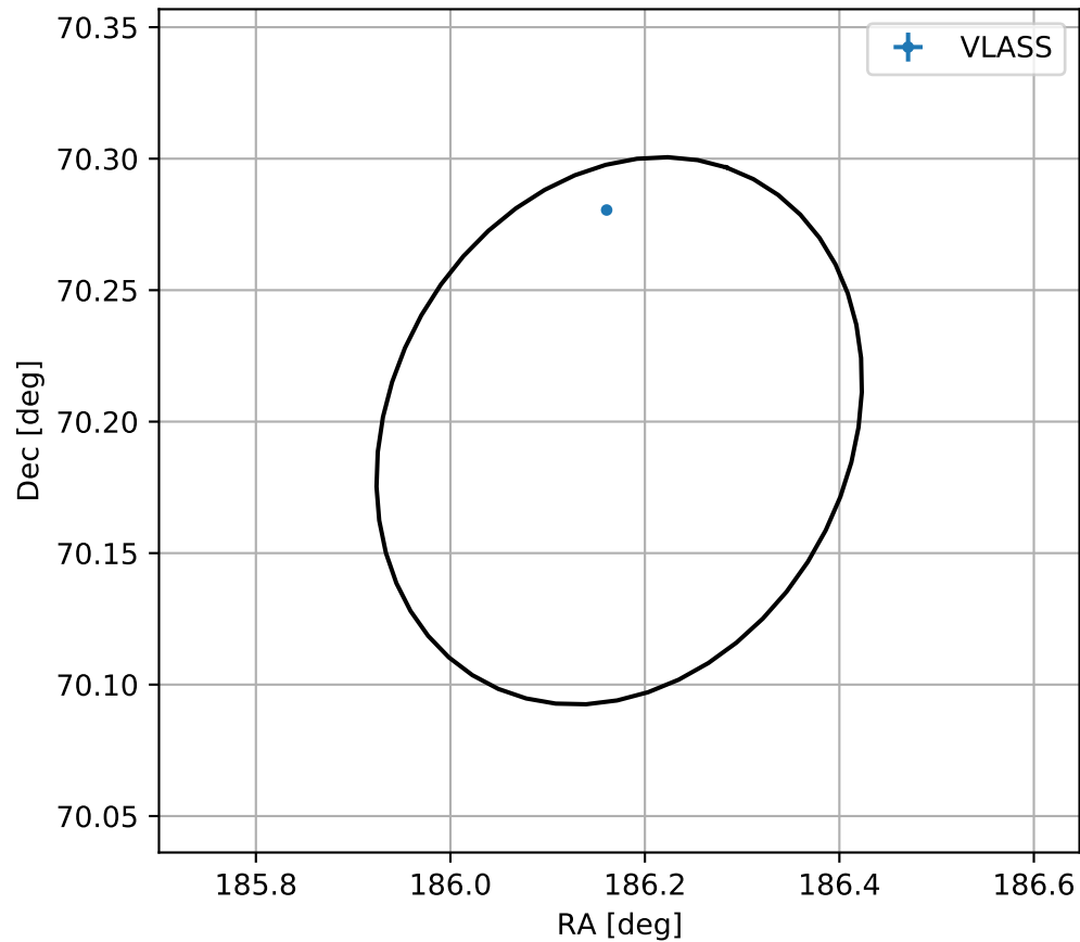
4FGL J1224.6+7011
