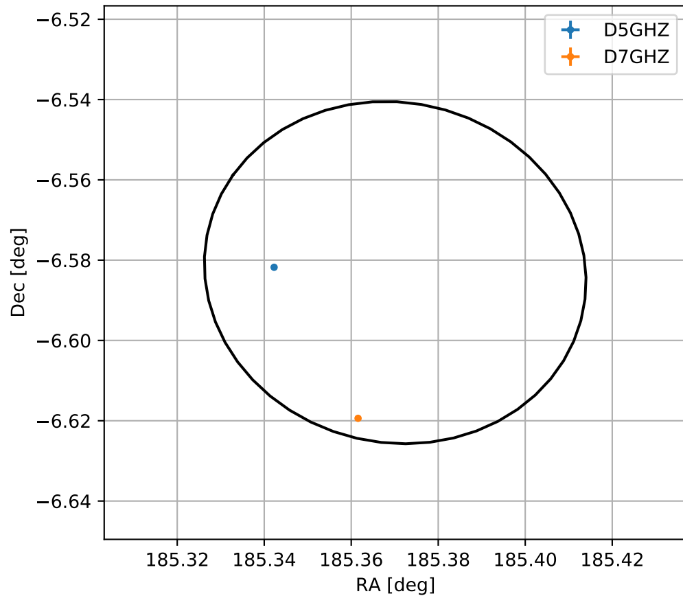
4FGL J1221.4-0634
